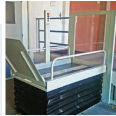
Optional: Door at upper landing with electric lock and a control pillar for public buildings
