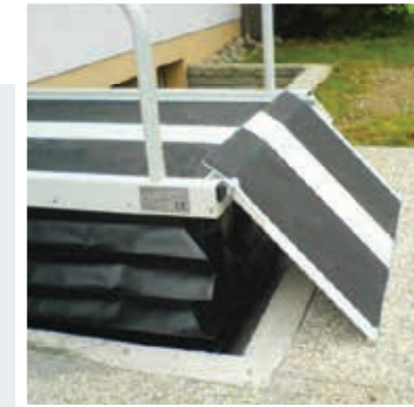
Optional: Manual access ramp folds down when unit is lifting and creates a barrier against rolling off
